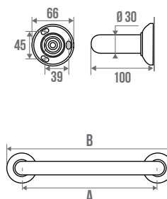
EMBASES INOX
